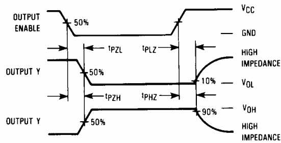
Figure 3. Switching Waveforms
