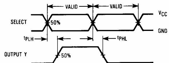
Figure 2. Switching Waveforms
