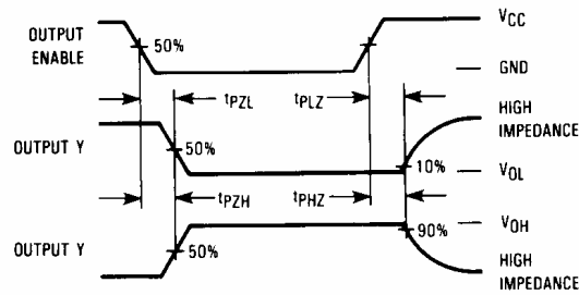
Figure 3. Switching Waveforms
