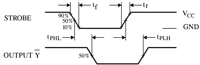
Figure 5. Switching Waveforms
