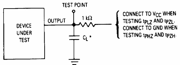
Figure 4. Test Circuit
